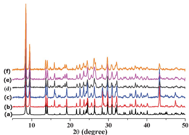
Fig. 3 PXRD pattern of compound 1 in different states. (a) simulated from single-crystal data; (b) as-synthesized \{[\text{Cu}_2(\text{pyzdc})] \cdot 0.83\text{H}_2\text{O}\}_n ; (c) dehydrated \{[\text{Cu}_2(\text{pyzdc})]\}_n ( 1' ); (d) rehydrated form of 1' ; (e) 1' exposed to the MeOH vapor and (f) 1' exposed to the MeCN vapor.
