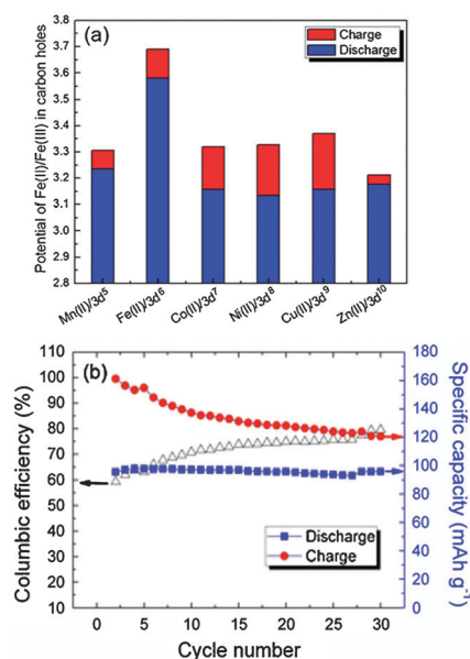
Fig. 4 (a) The redox potentials of the low-spin Fe(II)–Fe(III) in the Prussian blue compounds. (b) Cycling performance of KFe 2 (CN) 6 –Na battery cycled at C/20 between 2.0–4.0 V.
