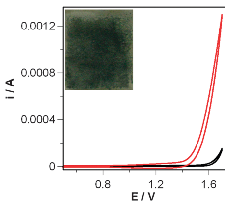
Fig. 1 Cyclic voltammograms of FTO slides ( R = 30 \text{ Ohm} \times \text{cm} ) coated by Nafion ® films only (blank, black curves) and Nafion/CoAPO5 films (red curves). Solution: 0.1 M \text{K}_2\text{SO}_4 in water. Scan rate 0.1 \text{ V s}^{-1} . 20 mg of catalyst was added on the slide dispersed in 0.3 mL of 5% w/w Nafion ® isopropanol solution. Inset: picture of the FTO/Nafion/CoAPO5 photoanode.
