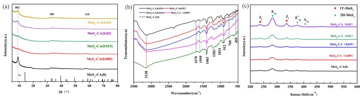
Fig. 3 (a) XRD patterns of \text{MoS}_2\text{-CA} , (b) FT-IR spectrum of \text{MoS}_2\text{-CA} , and (c) Raman spectra of \text{MoS}_2\text{-CA} .
