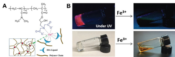
Fig. 7 (A) Schematic illustration and chemical structure of luminescent hydrogels with \text{Eu}^{3+} as the cross-linking points. (B) \text{Fe}^{3+} -induced luminescence quenching and gel-sol transition under UV light (upper) and daylight (lower). Reproduced with permission from ref. 67. Copyright: 2018, Wiley-VCH.
