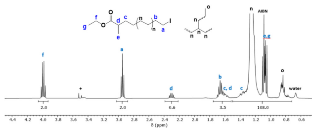
Fig. 2 ^1\text{H} NMR spectrum (in \text{TCE}/\text{C}_6\text{D}_6 at 90^\circ\text{C} ) of the PE synthesized at 70^\circ\text{C} , 80 bar in the presence of CTA-S1 after 3 h. “+” NMR solvent impurities. AIBN stands for the methyls from the chain-ends of the PE chains initiated by AIBN. The water is coming from the NMR solvent.
