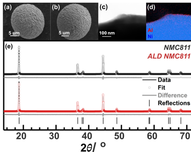
Fig. 1 SEM images of the as-synthesised (a) NMC811 and (b) the ALD NMC811 secondary particles (c) bright field image of an ALD NMC811 particle with (d) a corresponding EDX map of Ni (blue) and Al (red). The X-ray ( \lambda = 1.5406 \text{ \AA} ) diffraction patterns (e) of the NMC811 (black) and ALD NMC811 (red) are compared, showing the experimental data (solid line), the Rietveld refinement (open circles), the difference between the data and fit (grey line) and the position of the expected reflections of the R\bar{3}m space group (vertical ticks).
