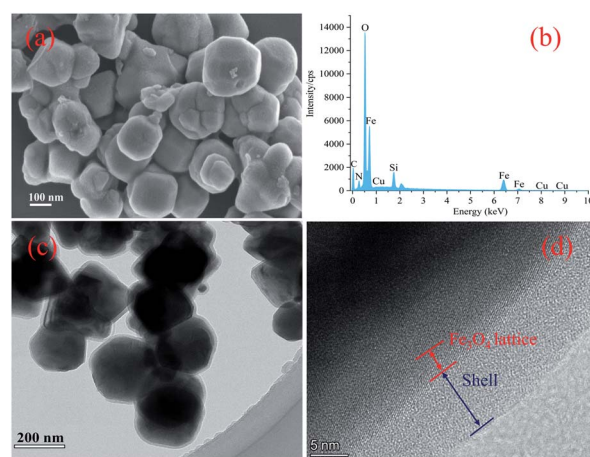
Fig. 1 SEM-EDS results of \text{Fe}_3\text{O}_4@ \text{SiO}_2@ \text{P}(\text{NIPAM-co-VI})/\text{Cu}^{2+} : (a) SEM image at 100 nm, (b) EDS spectrum (spot scanning); and TEM image of \text{Fe}_3\text{O}_4@ \text{SiO}_2@ \text{P}(\text{NIPAM-co-VI})/\text{Cu}^{2+} : (c) 200 nm, (d) 5 nm.
