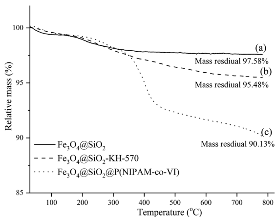
Fig. 4 TGA curves of the \text{Fe}_3\text{O}_4@SiO_2 (a), \text{Fe}_3\text{O}_4@SiO_2\text{-KH-570} (b), \text{Fe}_3\text{O}_4@SiO_2@P(\text{NIPAM-co-VI}) (c).
