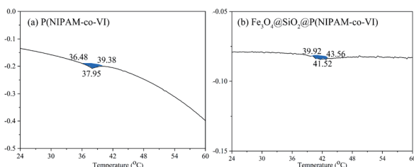
Fig. 5 DSC curves of P(NIPAM-co-VI) (a) and \text{Fe}_3\text{O}_4@SiO_2@P(\text{NIPAM-co-VI}) (b).
