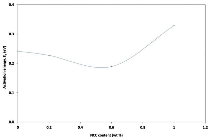
Fig. 5 Activation energy for the PEO-LI-NCC system.
