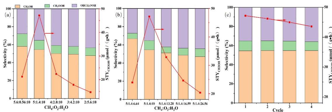
Fig. 9 (a) Effect of the molar ratio of CH_4 : O_2 on STY_{CH_3OH} and methanol selectivity of Cu(2)/MoO_3 . Reaction conditions: T = 600 °C. (b) Effect of the proportion of water on STY_{CH_3OH} and methanol selectivity of Cu(2)/MoO_3 . Reaction conditions: T = 600 °C. (c) Stability test of Cu(2)/MoO_3 . Reaction conditions: T = 600 °C, CH_4 : O_2 : H_2O = 5 : 1.4 : 10 .
