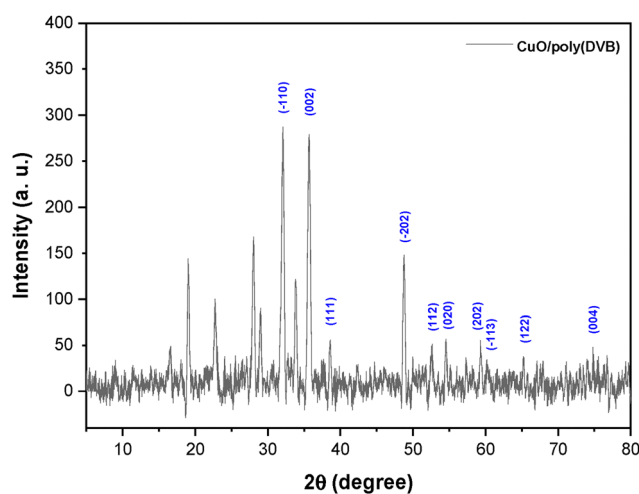
Fig. 5 XRD analysis of CuO/poly(DVB).
