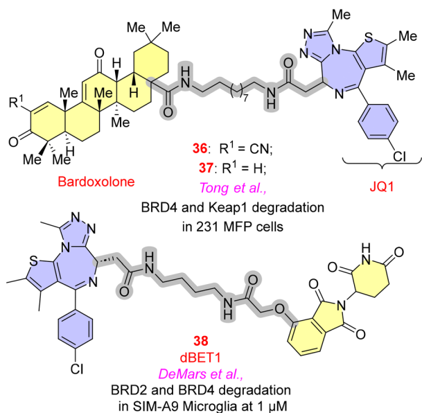
Fig. 10 BRD4-targeted PROTACs.
