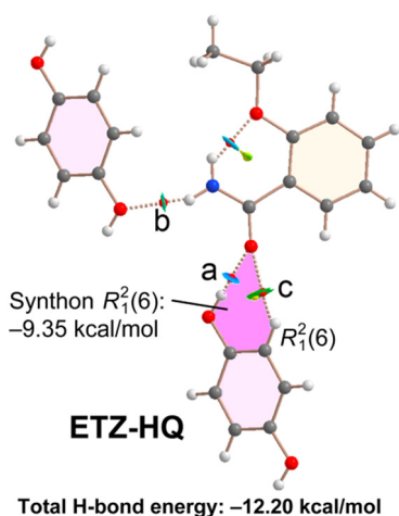
Fig. 10 Distribution of bond and ring critical points (red and yellow spheres, respectively) and bond paths in the H-bonding networks of ETZ-HQ. The overlapped NCIPlot index analysis is also shown. RDG isosurface 0.5 a.u., density cutoff = 0.04 a.u., color range: -0.04 \text{ a.u.} \leq \text{sign}(\lambda_2) \times \rho \leq 0.04 \text{ a.u.} For clarity, only the noncovalent interactions are represented in both QAIM and NCIPlot analyses.
