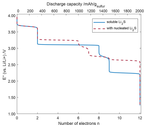
Fig. 6 Discharge curve of the cell potential vs. the number of electrons for soluble Li 2 S and nucleated Li 2 S.
