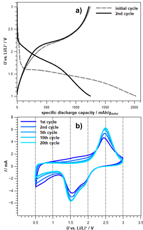
Fig. 7 Experimental (a) potential profile (0.2C) of the initial and second cycle and (b) cyclic voltammograms of exemplary cycles of Li-SPAN cells in a carbonate electrolyte. Electrolyte: 1 M LiPF 6 in DMC:EC (V:V = 1:1) + 10 wt% – FEC vs. Li/Li + . 66
