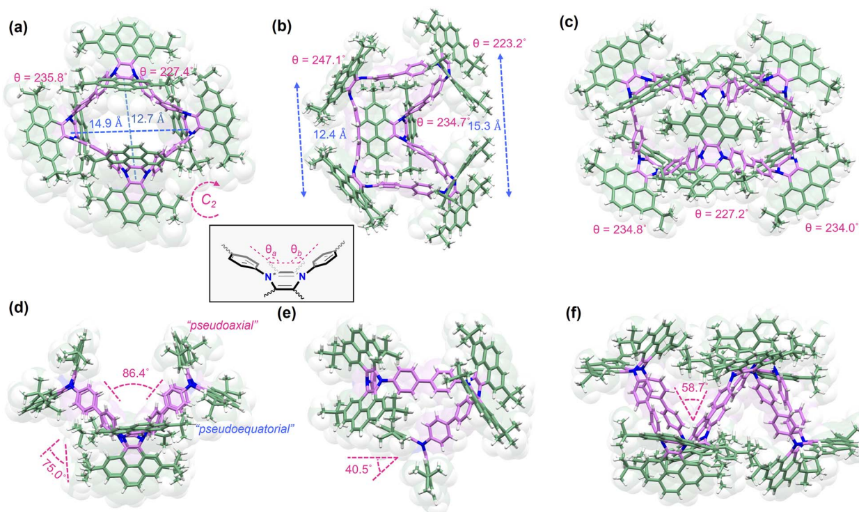
Fig. 2 X-ray crystallographic structures of DPP-Q (a: top view and d: side view), DPP-P (b: top view and e: side view), and DPP-H (c: top view and f: side view). Inset is an illustration of the bending angle in the dihydropyrazine corner.
