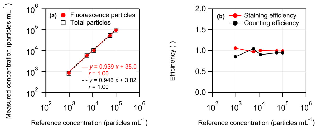
Fig. 7 Effect of particle number concentration (2 \mu m PS particles) on the swelling-mediated staining technique. (a) Reference concentration versus measured concentration for fluorescent particles and total particles. (b) Reference concentration versus staining and counting efficiencies.
