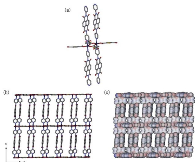
Fig. 1 Crystal structure of 1\supset\text{DMF} showing (a) coordination environment of Zn(II) ion and (b) pillared layer structure. Gray, blue, red, yellow, and navy are C, N, O, S and Zn, respectively. The hydrogen atoms and guest molecules are omitted for clarity. (c) VDW surface colored by the interpolated charge.
