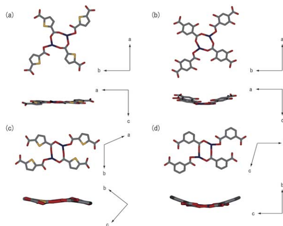
Fig. 3 Coordination environment of Zn(II) ion for (a) 1\supset\text{DMF} , (b) reported PCP; \{[\text{Zn}(\text{dhytpa})(\text{bpy})] \cdot 4\text{DMF}\}_n , (c) 2\supset\text{DMF} \cdot \text{MeOH} and (d) reported PCP; \{[\text{Zn}_2(\text{isa})_2(\text{bpy})_2] \text{DMF}\}_n .
