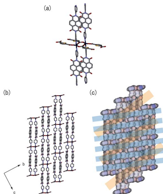
Fig. 2 Crystal structure of 2\supset\text{DMF} \cdot \text{MeOH} showing (a) coordination environment of Zn(II) ion and (b) 3D assembled framework with 2D layer structures. Gray, blue, red, yellow, and navy are C, N, O, S and Zn, respectively. The hydrogen atoms and guest molecules are omitted for clarity. (c) VDW surface colored by the interpolated charge. Blue and orange lines mean the intersecting linear pores.
