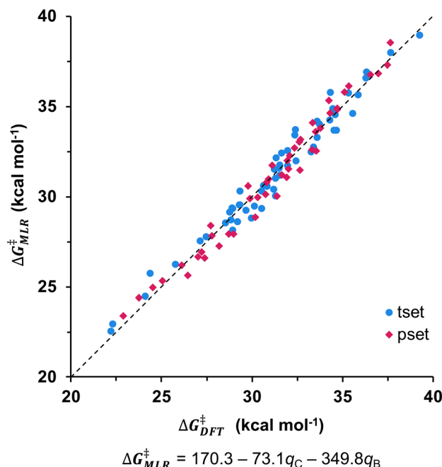
Fig. 5 \Delta G_{\text{MLR}}^{\ddagger} vs. \Delta G_{\text{DFT}}^{\ddagger} for the training and prediction sets of different substrate pairs.
