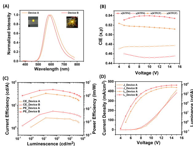
Fig. 10 (A) EL spectra of Devices A and B (inset: the image of real device illumination during operation). (B) CIE vs. voltage graph of Devices A and B. (C) Current efficiency–power efficiency–luminance curves of Devices A and B. (D) Current density–voltage–luminance curves of Devices A and B.
