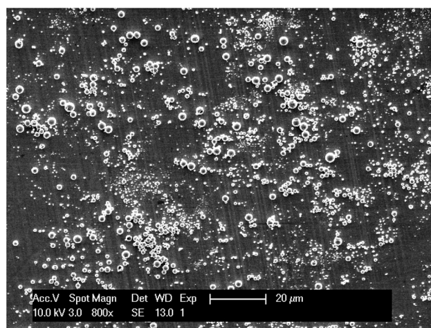
Fig. 11 SEM picture of indium deposited on a molybdenum working electrode at -2.00 \text{ V vs. Fc}^+/\text{Fc} at 180 °C for 2 h from purified Cyphos IL 101 loaded with 400 mM of indium(III) after supercritical drying.
