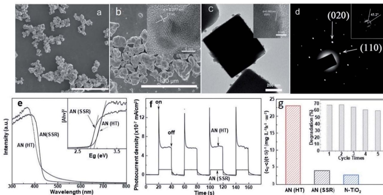
Fig. 48 Field-emission scanning electron microscopy images of \text{AgNbO}_3 (AN) prepared by (a) hydrothermal (HT) and (b) solid state (SSR) methods; (c) transmission electron microscopy image and (d) selected-area electron diffraction pattern of AN (HT); the insets in (b) and (c) show high-resolution transmission electron microscopy images of AN (SSR) and AN (HT), respectively; the inset in (d) shows the angle between the (020) and (110) facets in the AN (HT) cube; (e) UV-vis diffuse reflectance spectra of AN (HT) and AN (SSR); (f) transient photocurrent of AN (HT) and AN (SSR) irradiated with visible light ( \lambda \geq 400 nm); (g) specific photocatalytic activity of the catalysts. The inset in (g) shows repeated photocatalytic degradation of tetracycline in the presence of AN (HT) and nitrogen-doped \text{TiO}_2 , reported by Gao et al. 211 [Reproduced with permission from ref. 211 copyright 2019 by Elsevier].
