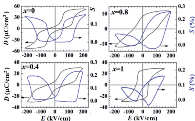
Fig. 33 P - E and S - E hysteresis loops of ANN solid-solution reported by Fu et al. 123 [Reproduced from ref. 123 https://doi.org/10.1063/1.3609234 with the permission of AIP Publishing].
