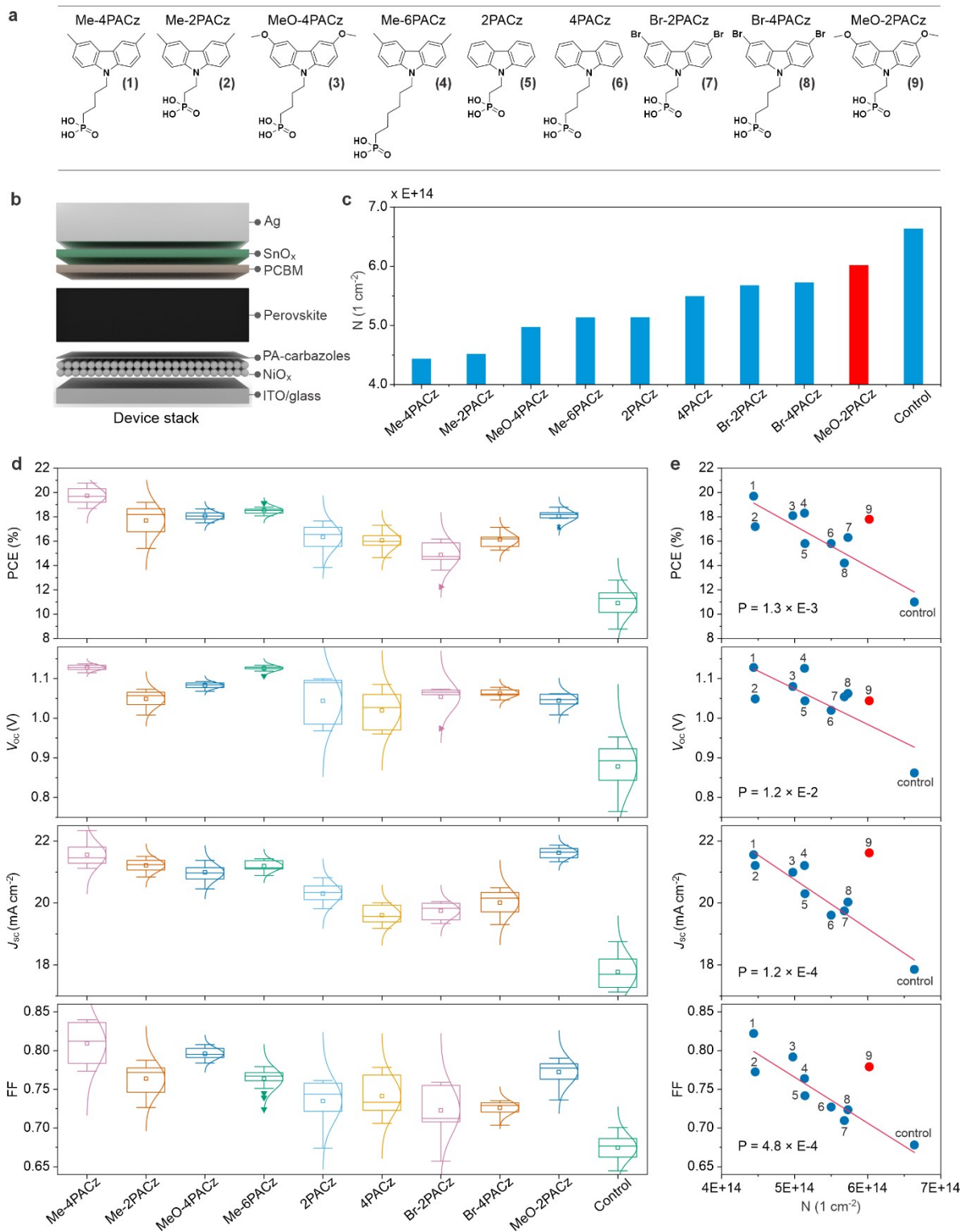
Fig. 3. PA carbazole passivation effects and their correlation to N -value
