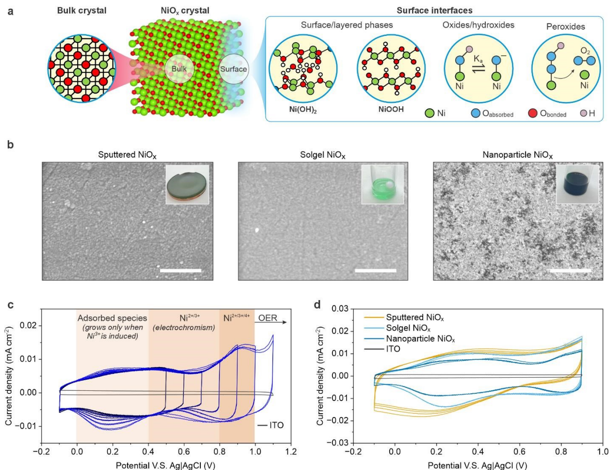
Fig. 1. NiO x films produced from sputtering, solgel or nanocrystal routes and their CV behavior.
