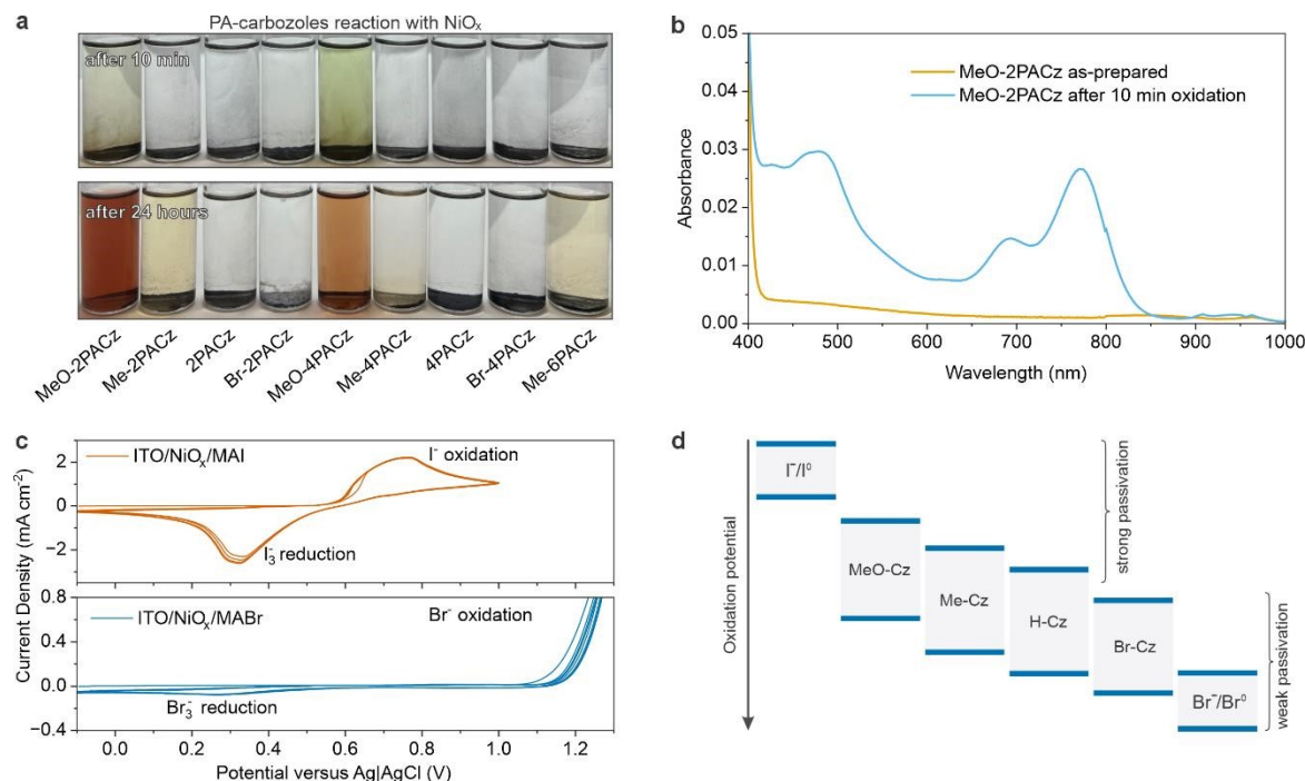
Fig. 5. PA carbazoles reaction and energy level comparison
