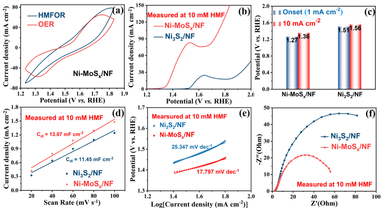
Fig. 5 (a) The first cyclic voltammograms of Ni-MoS x /NF with or without HMF in 1 M KOH solution. (b) Linear sweep voltammograms of Ni-MoS x /NF and Ni 3 S 2 /NF catalysts in 1 M KOH solution with 10 mM HMF. (c) Onset potential and the potential at 10 mA cm -2 . (d) Current density as a function of scan rate for the Ni-MoS x /NF and Ni 3 S 2 /NF catalysts. (e) Tafel plots and (f) Nyquist plots of Ni-MoS x /NF and Ni 3 S 2 /NF.
