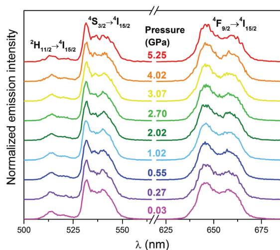
Fig. 6 Emission spectra of the \text{SrF}_2:\text{Yb}^{3+}, \text{Er}^{3+} sample under high pressure; \lambda_{\text{ex}} = 980 \text{ nm} , normalized to the {}^4\text{S}_{3/2} \rightarrow {}^4\text{I}_{15/2} band.
