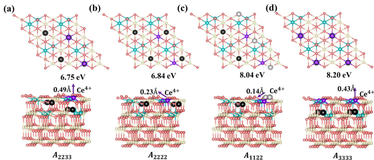
Fig. 4 Top views, side views, and the Vo's formation energies of the configurations A_{2233} , A_{2222} , A_{1122} and A_{3333} . (a) Configuration A_{2233} , with two V_O 's in the subsurface layer and two V_O 's in the 3 rd oxygen layer, (b) configuration A_{2222} , with four V_O 's in the subsurface layer, (c) configuration A_{1122} , with two V_O 's in the subsurface layer and two V_O 's in the surface layer and (d) configuration A_{3333} , with four V_O 's in the 3 rd layer. Ce^{4+} , Ce^{3+} , oxygen atoms and surface oxygen vacancies are depicted in white, blue, pink, and light gray, respectively; subsurface and third oxygen layer vacancies are depicted in black, and purple atoms are Ce^{4+} . Top and side views are depicted in the unrelaxed and relaxed states, respectively. The arrows indicate the relaxation direction of the purple-colored Ce^{4+} at the surface layer.
