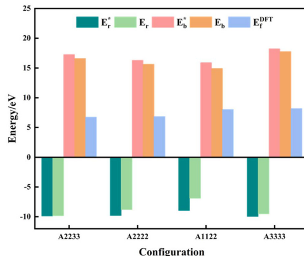
Fig. 5 Vacancy formation energy ( E_f^{DFT} ), relaxation energy ( E_r ), and bond-breaking energy ( E_b ) of the configurations with four V_O 's ( \theta = 1/4 ). E_r^* , E_b^* are the sum of the corresponding energies of isolated single V_O 's in the A_{mnpq} configurations.
