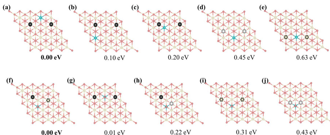
Fig. 3 Predicted relative energies of selected motifs of Vo's and \text{Ce}^{3+} s based on the identified 15 primary features. (a)–(e) the \text{Ce}^{3+} ion is located in the first cerium layer, (f)–(j) the \text{Ce}^{3+} ion is located in the second cerium layer. \text{Ce}^{4+} , \text{Ce}^{3+} , oxygen atoms, and surface oxygen vacancies are depicted in white, blue, pink, and light gray, respectively; subsurface and third oxygen layer vacancies are depicted in black. Structures are depicted in the unrelaxed state.
