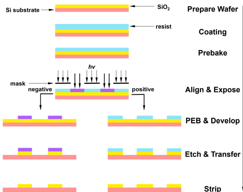
Fig. 2 The typical photolithography process.
