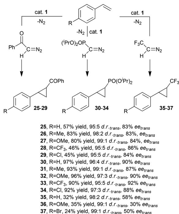
Scheme 7 Complex 1-catalysed synthesis of cyclopropylketones 25–29, 31 trans -cyclopropylphosphonates 30–34 32 and trifluoromethylphenyl cyclopropanes 35–37. 33
