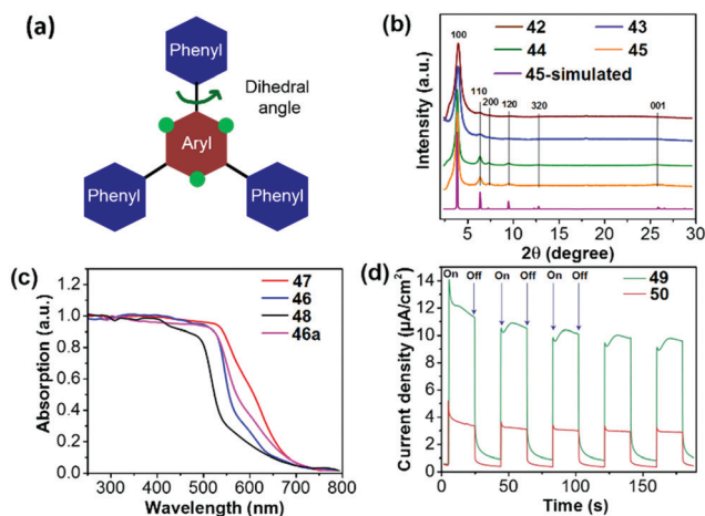
Fig. 11 (a) Design principle and (b) PXRD patterns of COFs 42–45 . (c) Diffuse reflectance spectra of COFs 46–48 ( 46a is an amorphous analogue of 46 ). (d) Transient photocurrent for COFs 49 and 50 measured in 0.5 M KCl solution under visible light irradiation. Reprinted with permission from ref. 120–122. Copyright 2015 Nature Publishing Group, 2018 Nature Publishing Group and 2018 American Chemical Society.
