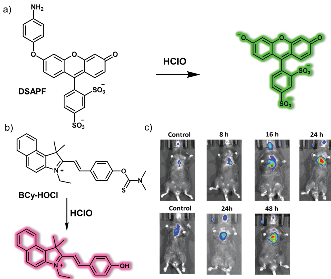
Fig. 30 Chemical structure of small molecule-based fluorescent probes, (a) DSAPF , (b) BCy-HOCl , and a working model showing how they may be used to detect \text{HClO} . (c) Time-dependent fluorescence images of the LPS (top) and hyperoxia (bottom)-induced ALI mice administered intratracheally with BCy-HOCl . \lambda_{\text{ex}} = 543 \text{ nm} , \lambda_{\text{em}} = 600\text{--}700 \text{ nm} . n = 5 . Reproduced with permission from ref. 45. Copyright (2020) The Royal Society of Chemistry.
