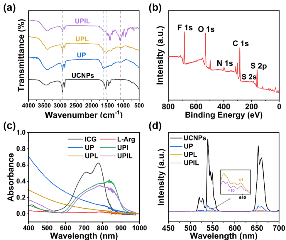
Fig. 2 Characterization of the as-prepared nanoparticles. (a) FT-IR spectra of UCNPs, UP, UPL, and UPIL. (b) X-ray photoelectron spectroscopy (XPS) of UPIL. (c) UV-vis-NIR absorbance spectra of ICG, L-Arg, UP, UPI, UPL, and UPIL, respectively. (d) Upconversion luminescence spectra (under an excitation of 980 nm) of UCNPs, UP, UPL, and UPIL, respectively.
