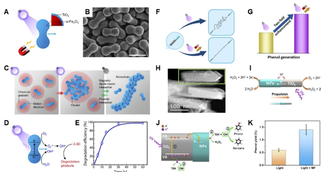
Fig. 2 Design, structure, and photocatalytic performance of TiO 2 /α-Fe 2 O 3 microrobots and TiO 2 /NiFe nanomotors. (A) Schematic illustration of TiO 2 /α-Fe 2 O 3 microrobots with light- and magnetically driven motion. (B) SEM image of peanut-shaped α-Fe 2 O 3 particles, scale bar 2 μm. (C) Self-assembly behaviour under chemical gradients and magnetic dipole–dipole interactions forming clusters and microchains. (D) Photocatalytic mechanism of dichlorophenoxyacetic acid (2,4-D) degradation via ROS generation mediated by UV light. (E) Graph showing time-dependent degradation efficiency of 2,4-D, reaching 97% in 30 minutes. Adapted with permission from Nature Communications , ref. 48 Copyright©2023. This is an open access article distributed under the terms of the Creative Commons CC BY license. (F) Schematic illustrating the motion behaviour of TiO 2 /NiFe nanomotors under UV light and magnetic fields. (G) Representation of improved photocatalytic phenol generation by the combined effects of light and magnetic fields. (H) STEM image of TiO 2 /NiFe nanomotors. (I) Photocatalytic propulsion mechanism of TiO 2 /NiFe nanomotors mediated by UV light, driven by electron transfer and H 2 O 2 decomposition. (J) UV light-induced electron excitation in TiO 2 and charge transfer to NiFe, generating ROS that oxidize benzene to phenol. (K) Phenol yield comparison under light and light + magnetic field conditions, showing enhanced performance. Reprinted with permission from ACS Applied Materials & Interfaces , ref. 50 (ACS) Copyright©2023. ( https://pubs.acs.org/doi/10.1021/acsami.4c03905 ). Readers are advised that any requests for additional permissions relating to the extracted material must be addressed directly to ACS.
