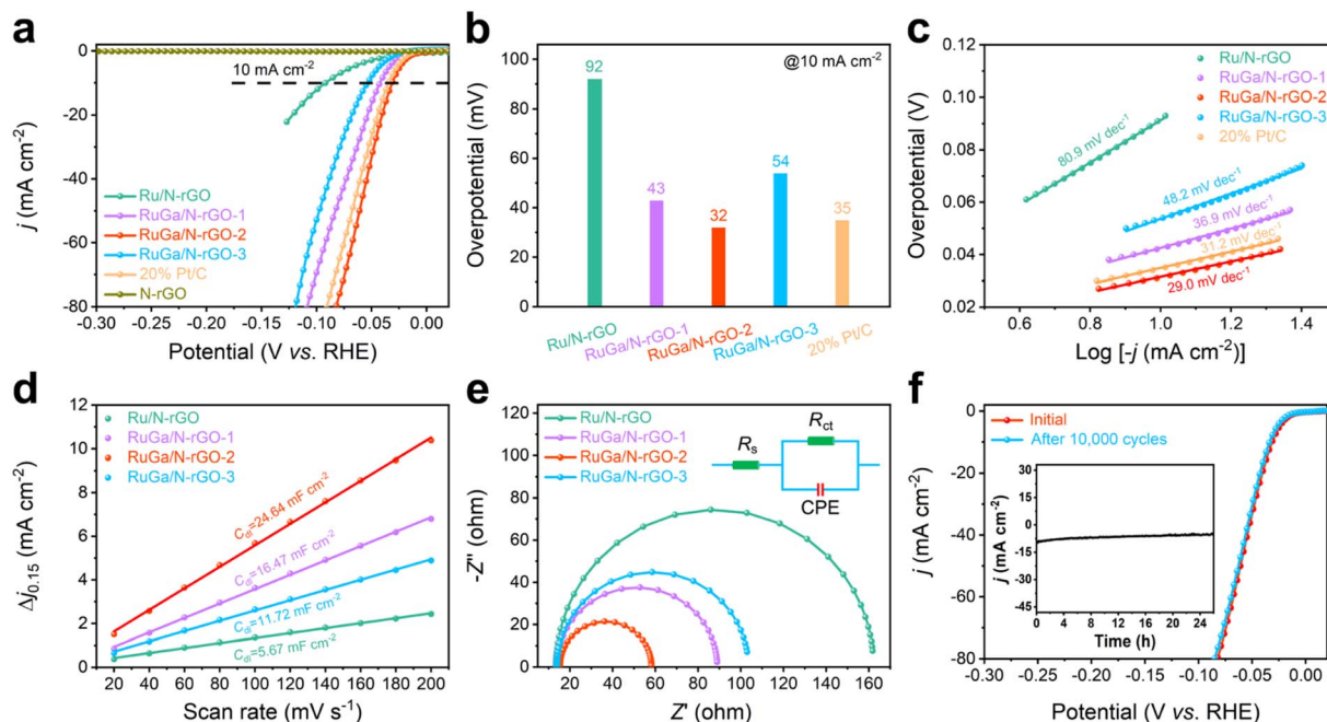
Fig. 3 (a) LSV curves of RuGa/N-rGO- n ( n = 1, 2, 3), Ru/N-rGO, commercial Pt/C, and pure N-rGO towards acidic HER. (b) The histograms of overpotential values taken from the current density of 10 mA cm -2 . (c) The corresponding Tafel plots obtained from (a). (d) The calculated values of C dl . (e) Nyquist plots measured at -0.03 V (inset: the related equivalent circuit for fitting the Nyquist plots). (f) LSV curves over RuGa/N-rGO-2 before and after the accelerated degradation tests (inset: chronoamperometric curve of RuGa/N-rGO-2 recorded at the constant overpotential of 30 mV for 26 hours).
