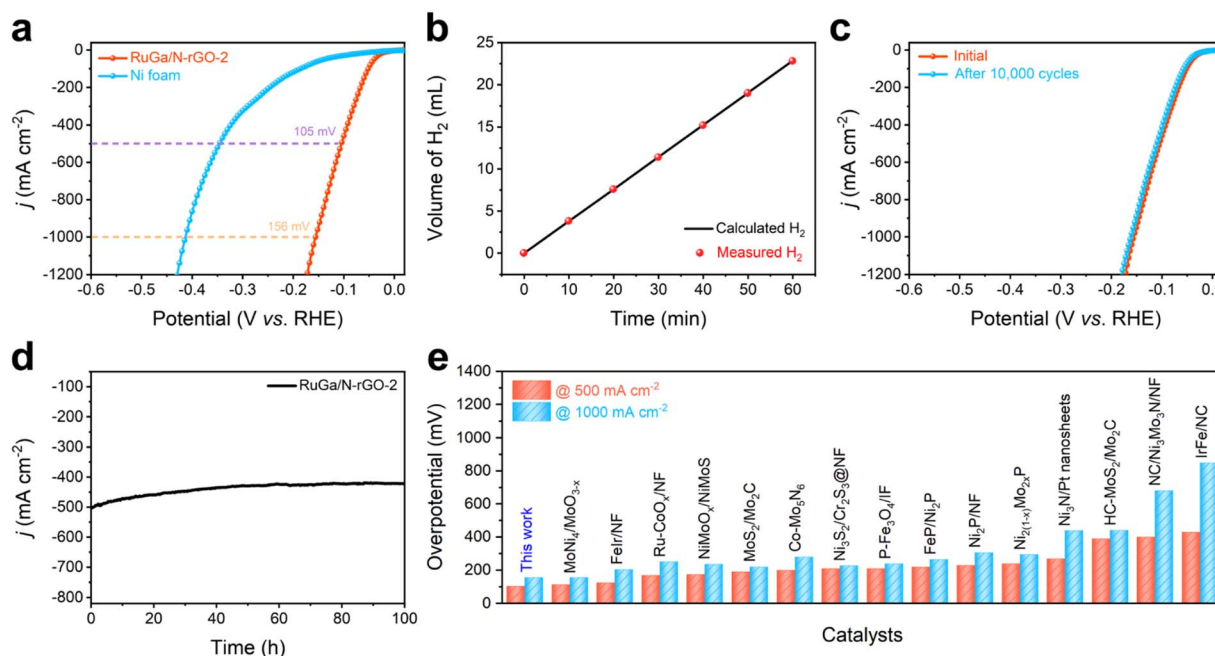
Fig. 5 (a) LSV curves of RuGa/N-rGO-2 and pure Ni foam for large-current-density HER in 1.0 M KOH electrolyte. (b) Theoretically calculated and experimentally measured \text{H}_2 gas amounts versus time over RuGa/N-rGO-2. (c) LSV curves for RuGa/N-rGO-2 before and after the accelerated degradation tests. (d) Chronoamperometric curve of RuGa/N-rGO-2 at the constant overpotential of 100 mV for 100 hours. (e) The comparison of overpotential values obtained at 500 and 1000 \text{ mA cm}^{-2} between RuGa/N-rGO-2 and some reported electrocatalysts.
