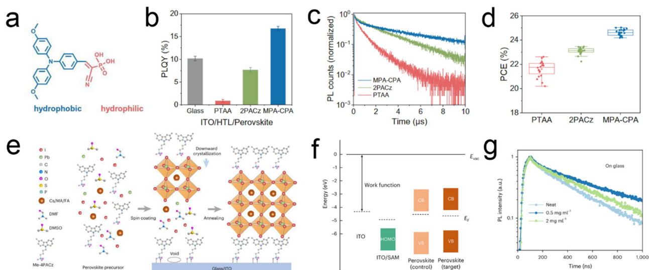
Fig. 7 (a) Molecular structure of the amphoteric MPA-CPA molecule. (b) PL quantum yield and (c) PL decays of perovskite films on different substrates. (d) The statistics of PCE values for devices based on different HTLs. Reproduced with permission. 62 Copyright 2023, Science Publishing Groups. (e) Illustration of SAM formation and the perovskite crystallization process. (f) Energy-level diagram. (g) TRPL of perovskite films with different concentrations of Me-4PACz on glass substrates. Reproduced with permission. 13 Copyright 2022, Nature Publishing Groups.
