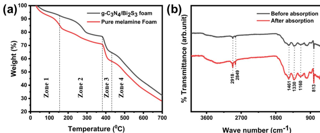
Fig. 5 (a) TGA for the g\text{-C}_3\text{N}_4/\text{Bi}_2\text{S}_3 foam and pure melamine foam. (b) FTIR spectra of g\text{-C}_3\text{N}_4/\text{Bi}_2\text{S}_3 foam before and after absorption.
