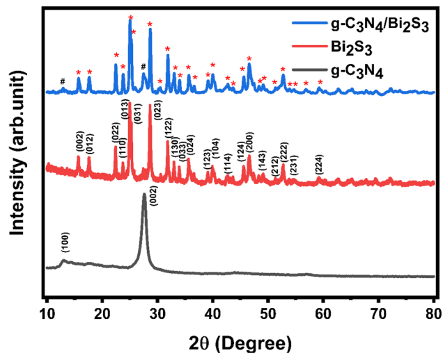
Fig. 2 XRD patterns of synthesized g\text{-C}_3\text{N}_4 , \text{Bi}_2\text{S}_3 , and g\text{-C}_3\text{N}_4/\text{Bi}_2\text{S}_3 nanocomposite.
