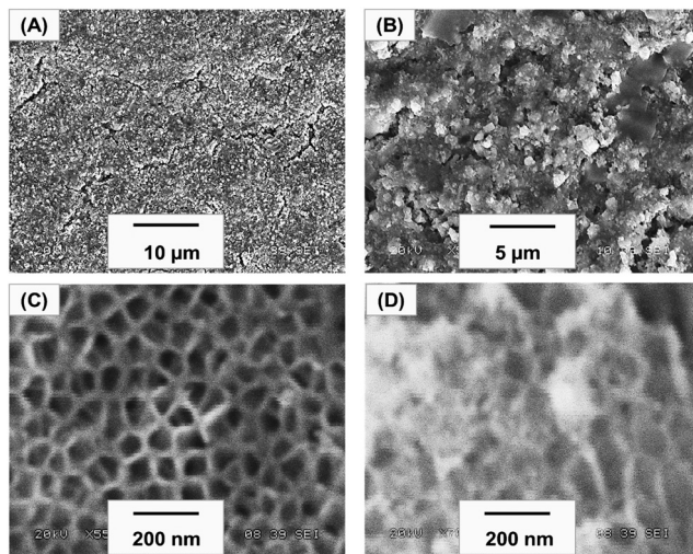
Fig. 3 SEM image of (A) and (B), the as-synthesized biogenic Ag-NPs at low (×1000) and high magnifications (×5000); (C) and (D), anodized aluminum (AAO/Al) and biogenic Ag-NP coated anodized aluminum (Ag/AAO/Al) coupon, respectively.
