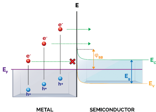
Fig. 3 Schematic illustration of the metal/semiconductor Schottky barrier. Upon excitation, only hot electrons with enough energy can surpass the Schottky barrier ( \phi_{SB} ) and transfer into the conduction band of the semiconductor.
