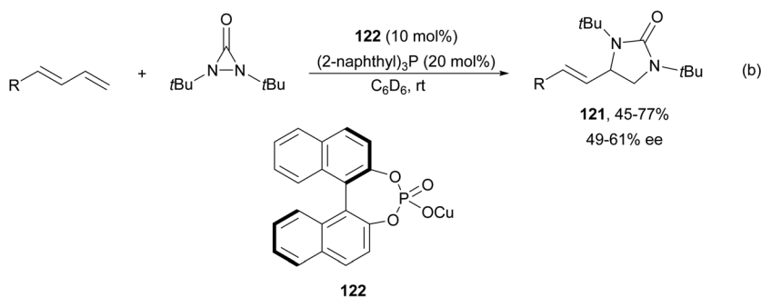
Scheme 43 Asymmetric radical intermolecular diamination of conjugated dienes under Cu(I) catalysis.
