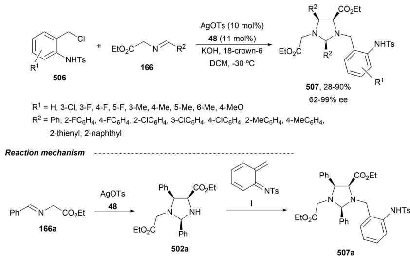
Scheme 153 Asymmetric tandem 1,3-DC/1,4-addition of imino esters 166 with N -tosyl- o -(chloromethyl)anilines 506 under AgOTs/ferrocenylphosphine 48 catalysis.
