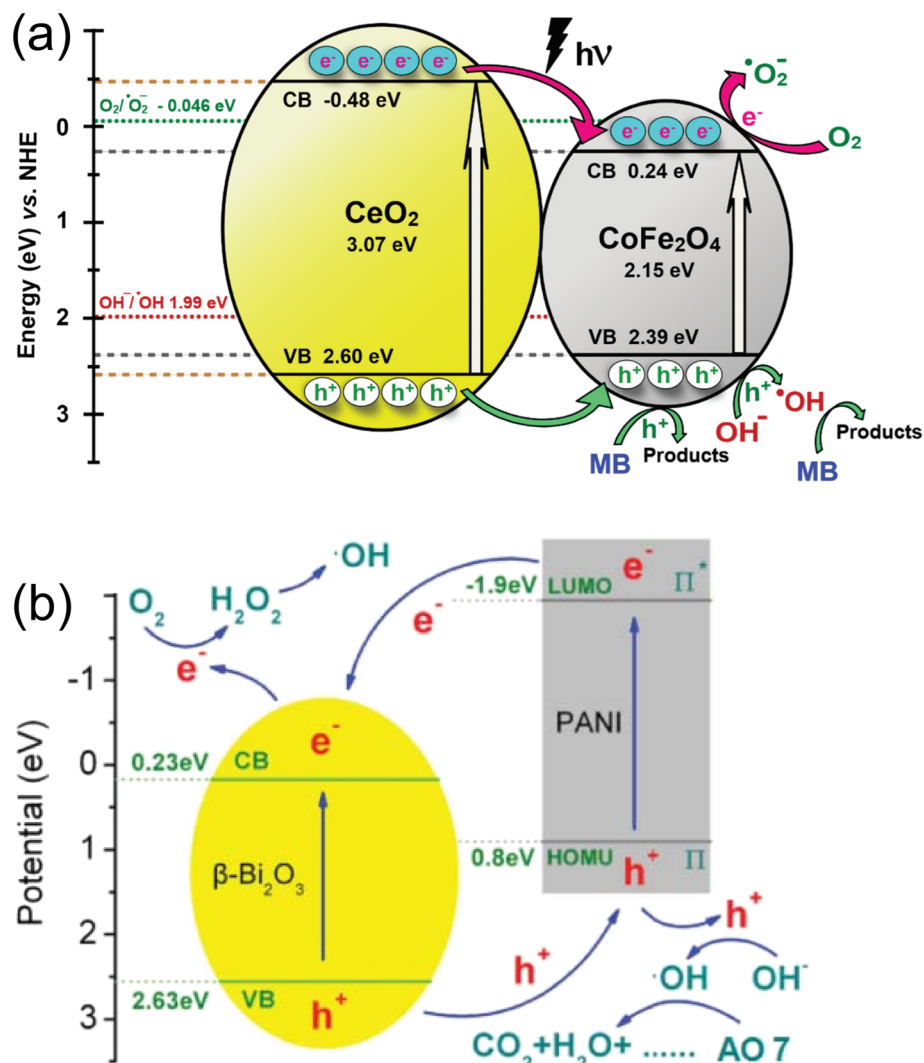
Fig. 5 (a) Schematic illustration of the heterojunction configuration in the \text{CeO}_2/\text{CoFe}_2\text{O}_4 system. Reprinted with permission. 49 Copyright 2024, Taylor & Francis. The proposed configuration in the polyaniline/ \beta\text{-Bi}_2\text{O}_3 heterojunction is shown in panel (b). Reprinted with permission. 50 Copyright 2017, Taylor and Francis.
