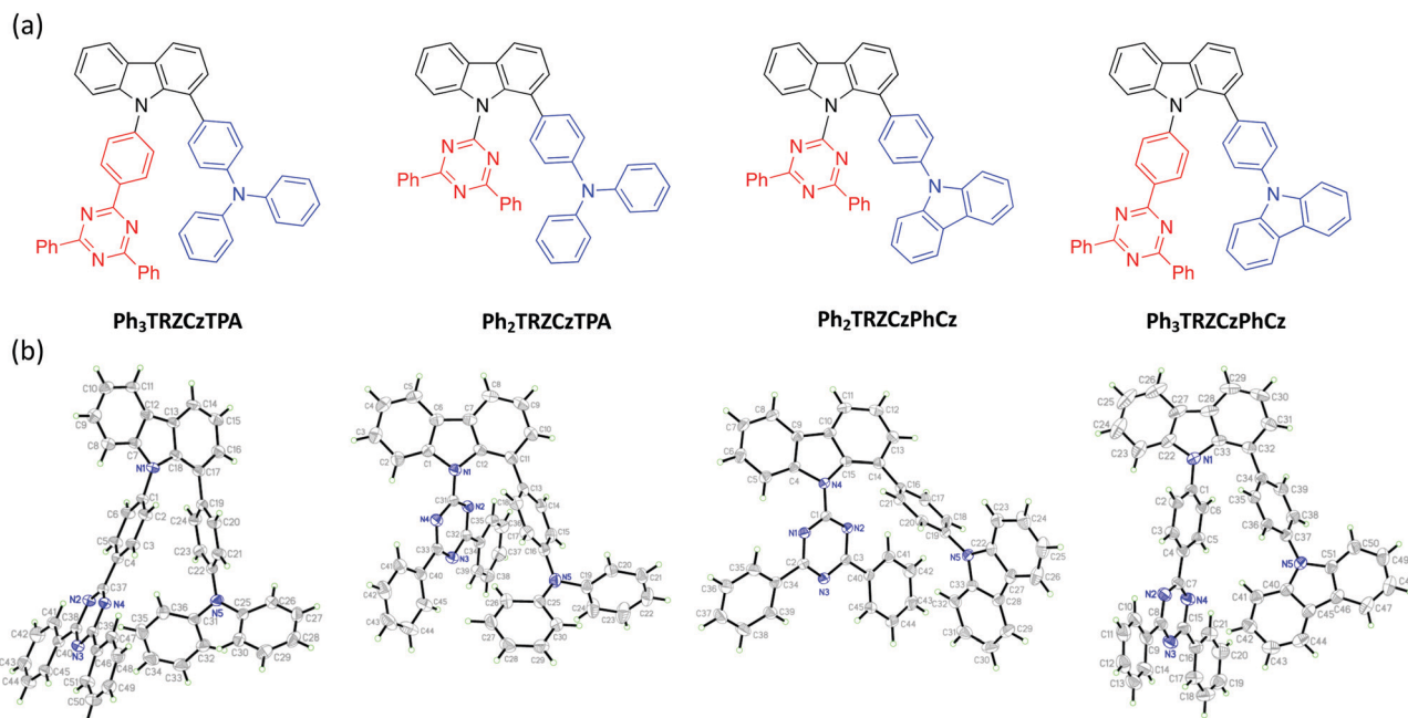
Fig. 1 The chemical structures (a) and X-ray structures (b) of Ph 3 TRZCzTPA , Ph 2 TRZCzTPA , Ph 2 TRZCzPhCz and Ph 3 TRZCzPhCz , thermal ellipsoids were drawn at a 50% probability level.
