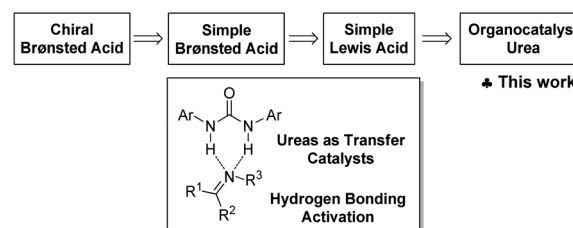
Scheme 1 Biomimetic asymmetric reduction (BMAR) based on the coenzyme NAD(P)H and transfer catalysts.
