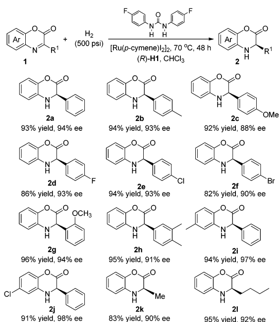
Scheme 2 The BMAR of benzoxazinones. Reaction conditions: 1 (0.20 mmol), [Ru( p -cymene) I_2 ] _2 (0.5 mol%), ( R )- H1 (10 mol%), OC- 3 (20 mol%), CHCl _3 (3 mL), H _2 (500 psi), 70 °C, and 48 h.
