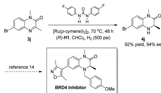
Scheme 4 The BMAR of bromine-substituted quinoxalinone and synthesis of a key intermediate of a BRD4 inhibitor.
