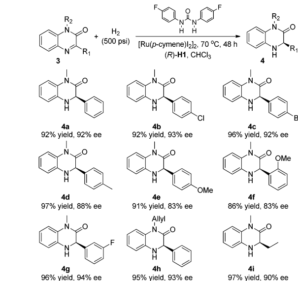
Scheme 3 The BMAR of quinoxalinones. Reaction conditions: 3 (0.20 mmol), [Ru( p -cymene) I_2 ] _2 (0.5 mol%), ( R )- H1 (10 mol%), OC- 3 (20 mol%), CHCl _3 (3 mL), H _2 (500 psi), 70 °C, and 48 h.
