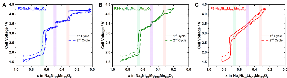
Fig. 11 Potential profile for the first two full galvanostatic cycles of (A) \text{P2-Na}_{2/3}\text{Ni}_{1/3}\text{Mn}_{2/3}\text{O}_2 , (B) \text{P2-Na}_{2/3}\text{Ni}_{1/4}\text{Mg}_{1/12}\text{Mn}_{2/3}\text{O}_2 and (C) \text{Na}_{3/4}\text{Ni}_{1/4}\text{Li}_{1/12}\text{Mn}_{2/3}\text{O}_2 as cathode materials in a sodium half-cell.
