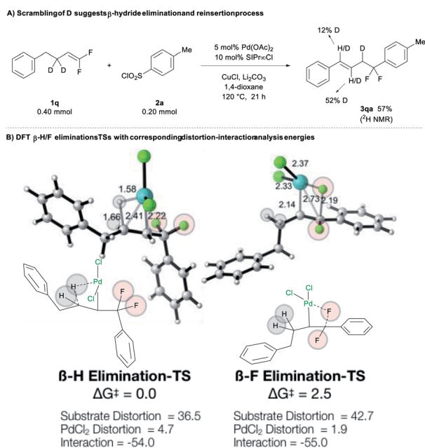
Fig. 2 Calculated β-H/F elimination transition states (TSs) with corresponding distortion-interaction analysis energies. Distances in Å and energies in kcal mol -1 .
