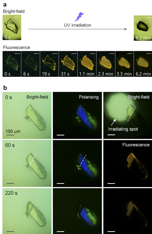
Fig. 2 Photographic images of the photoinduced crystal melting with luminescence evolution observed under microscope. (a) Whole crystal was exposed to UV irradiation (scale bar: 50 μm). (b) Top-left part of the crystal was exposed to UV irradiation. Polarising optical microscope images were taken under cross Nichol prism.
