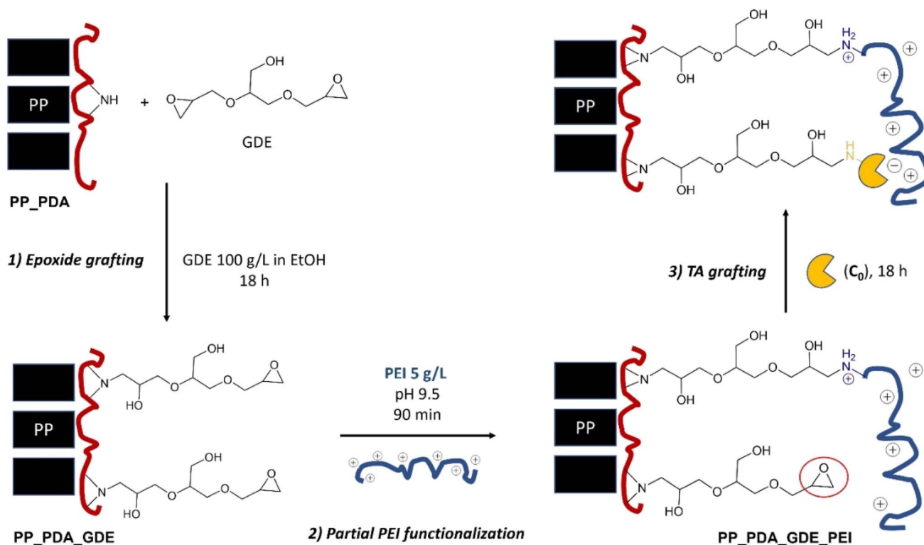
Fig. 2 Schematic representation of PP_PDA functionalization and TA immobilization procedures on PP-based membranes, leading to TA_PPY catalysts. In some cases, the protocole was modified by adding an additional step ( i.e. PLP immobilization) after the third step.
