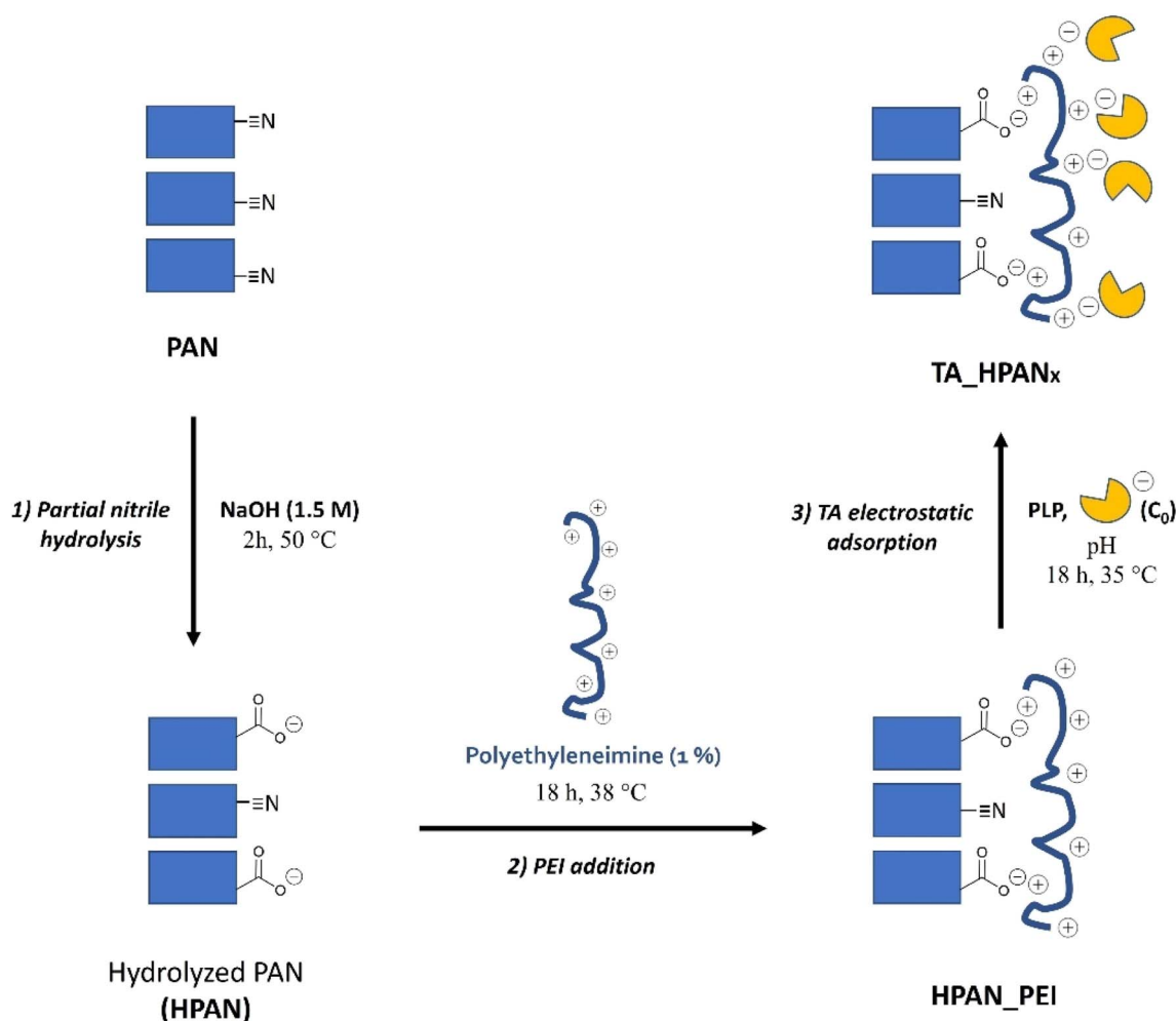
Fig. 1 Schematic representation of PAN functionalization and TA immobilization procedures, leading to \text{TA\_HPAN}_{\text{xa}} or \text{TA\_HPAN}_{\text{xb}} . In the case of \text{TA\_HPAN}_{2\text{a}} , \text{TA\_HPAN}_{2\text{b}} , \text{TA\_HPAN}_{3\text{a}} and \text{TA\_HPAN}_{3\text{b}} , an additional post-treatment was applied (with SA or GA, respectively) before the rinsing step.
