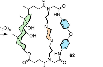
Fig. 12 Kinetically stable organic cages can be prepared via a variety of methodologies and using myriad reactions. R groups omitted from SCXR structures for clarity.
