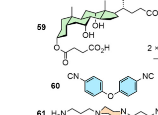
Fig. 12 Kinetically stable organic cages can be prepared via a variety of methodologies and using myriad reactions. R groups omitted from SCXR structures for clarity.
