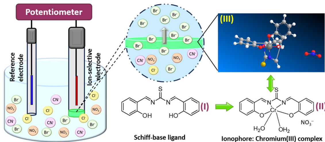
Fig. 1 The components and selective mechanism for bromide ions by using a potentiometric method, with the Cr(III) salicylidene Schiff base complex as an ionophore. Inset: CrC and salicylidene Schiff base prepared in one-pot preparation (I), coordination environment of Cr(III) in the complex CrC, and simulated configuration of the CrC coordination complex.
