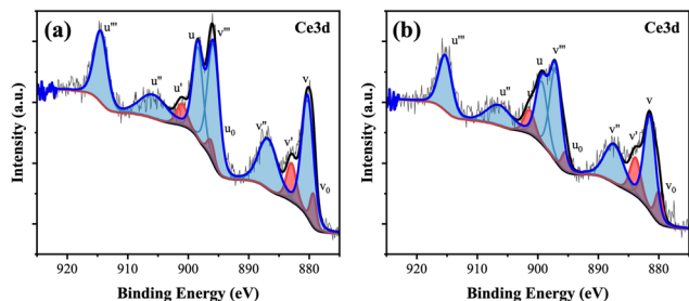
Fig. 5 XPS results for Ce 3d of (a) CeO 2 and (b) 0.9CeO 2 @0.1ZrO 2 .
