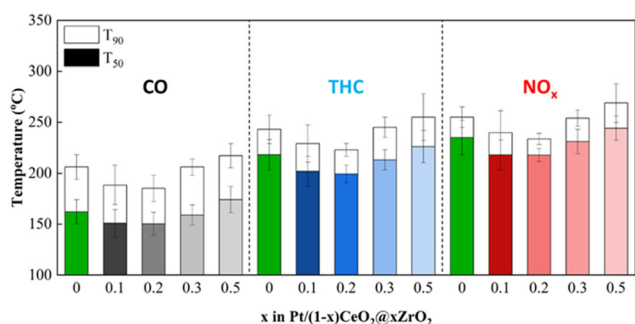
Fig. 6 Comparison of T_{50,90} s of CO, THCs and NO x over DG 1.8 wt% Pt/(1 - x)CeO 2 @xZrO 2 (x = 0, 0.1, 0.2, 0.3, 0.5) catalysts; each bar represents the average T_{50,90} s of three different batches of the catalyst and the error bars represent the standard deviation of the T_{50,90} s.
