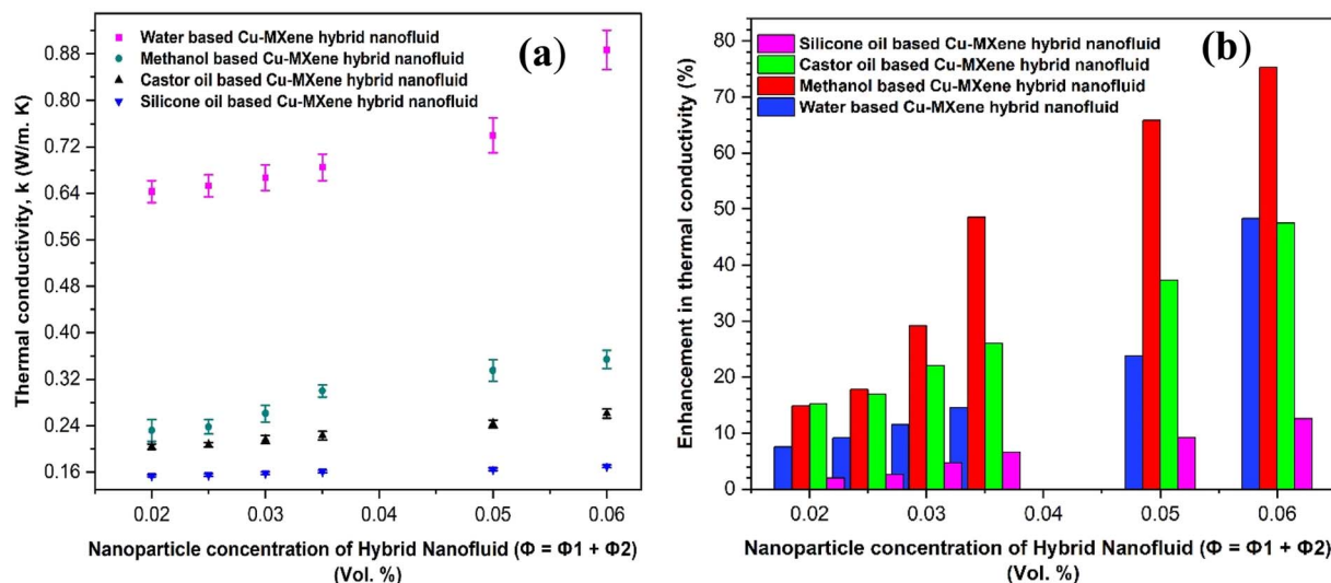
Fig. 17 Effect of concentration of MXene nanostructures on (a) thermal conductivity of base fluids and (b) the enhancement of thermal conductivity in hybrid nanofluids.
