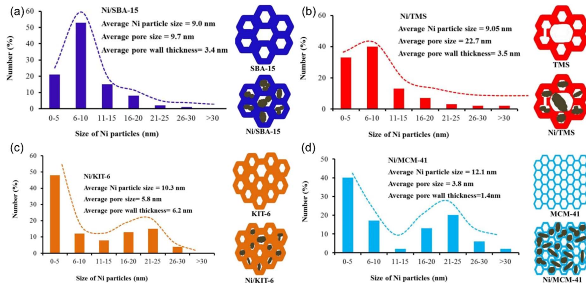
Fig. 14 Structural properties of different mesoporous silica supports. (a) Ni/SBA-15, (b) Ni/TMS, (c) Ni/KIT-6, (d) Ni/MCM-41. Reproduced with permission from ref. 143 Copyright 2020, MPDI.
