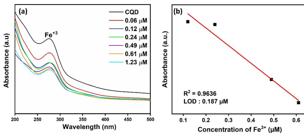
Fig. 5 (a) UV-vis spectra of CQDs at different \text{Fe}^{3+} concentrations and (b) linear calibration curves of the absorption intensity of CQDs at different \text{Fe}^{3+} concentrations.
